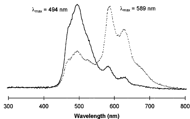
Figure 4. Electrogenenerated chemiluminescence of stirred (—) and unstirred (---) 0.24 mM solutions of 2 in benzene/acetonitrile (1:1; 0.3 M TBAPF 6 ; 1 Hz cycling between +1.55 and -1.80 mV).
