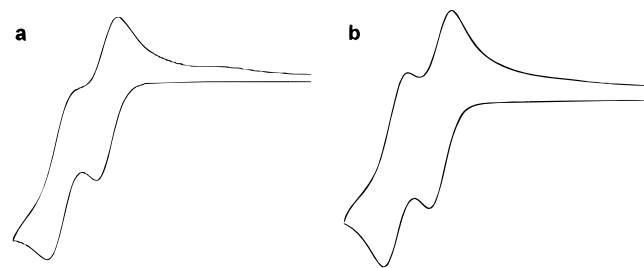
Figure 2. Cyclic voltammograms of the oxidation of 2 at (a) 50 mV/s and (b) 500 mV/s in benzene/acetonitrile (1:1; 0.3 M TBAPF 6 ).
