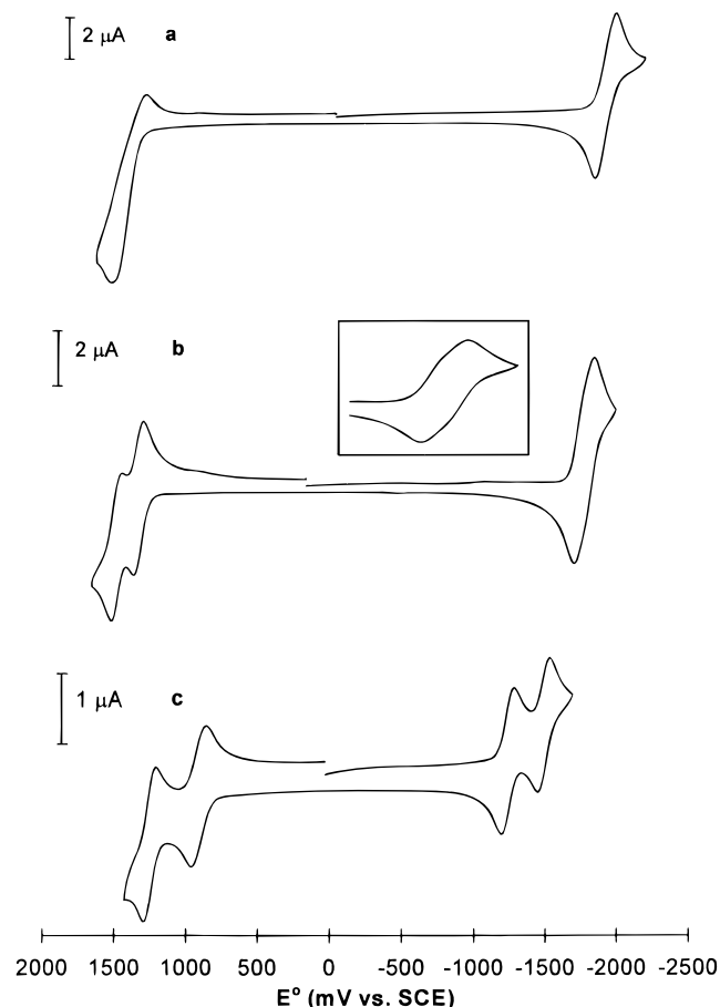
Figure 1. Cyclic voltammograms of (a) 1.5 mM 1 , (b) 0.56 mM 2 , and (c) 0.31 mM 3 in benzene/acetonitrile (1:1; 0.3 M TBAPF 6 ), scan rate 100 mV/s. The reduction wave of 2 is shown in the inset at a scale that more clearly illustrates the dual nature of the reduction.
